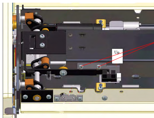
Top Position Sensor fixing screws
